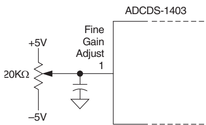
Figure 5. Fine Gain Adjustment Circuit
