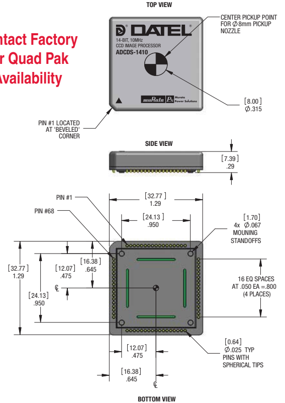
Quad Pak
