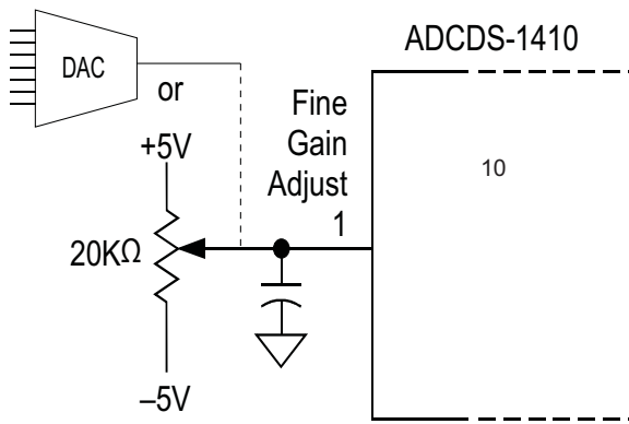
Figure 5. Fine Gain Adjustment Circuit
