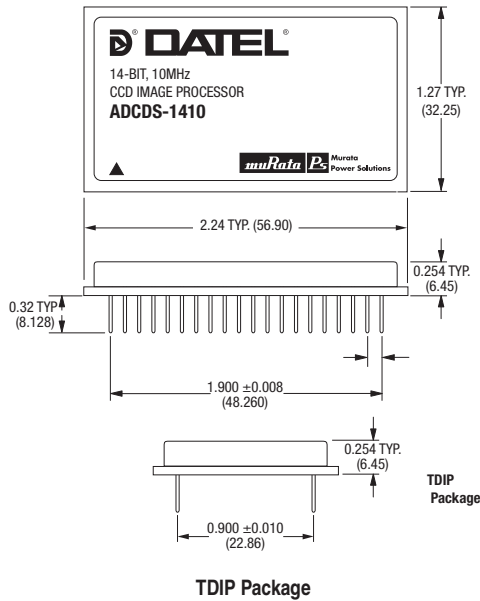
TDIP Package
