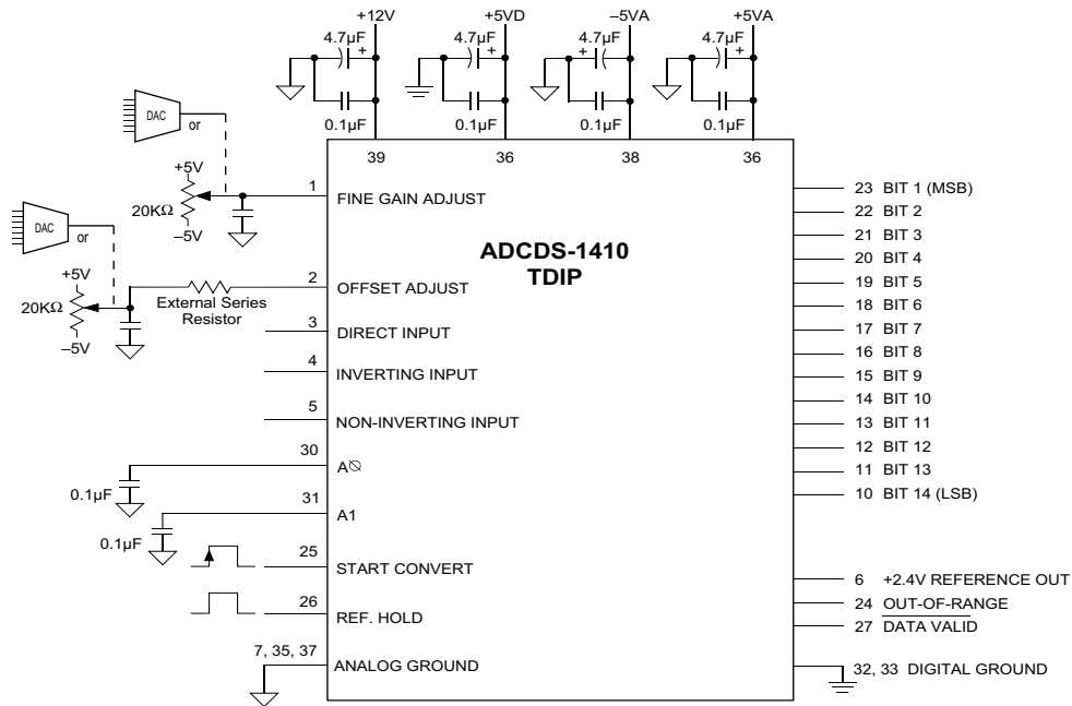
Figure 9a. ADCDS-1410 TDIP Connection Diagram
