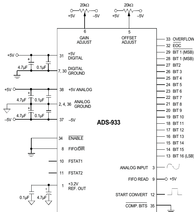
Figure 2. Bipolar Connection Diagram
