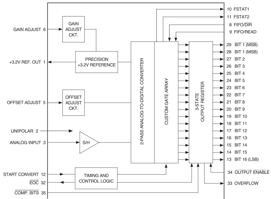
Figure 1. ADS-935 Functional Block Diagram
