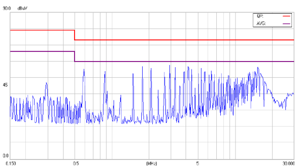
Class A conducted Line test for QB22S28-5.4
