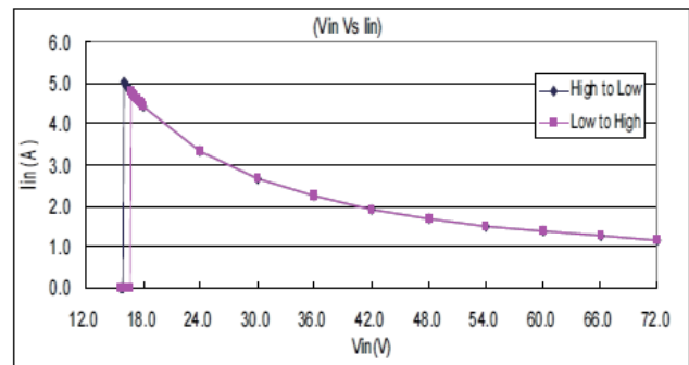
QB45SXX series I in vs V in
