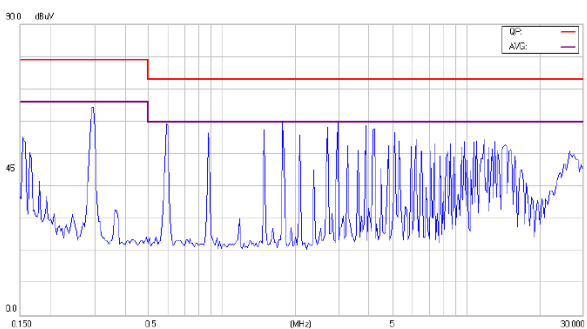
Class A conducted Line test for QB22S24-6.3
