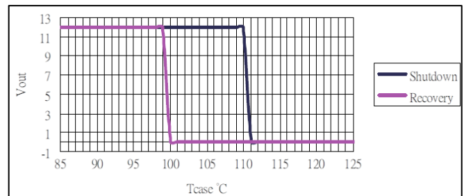
Shutdown and Recovery Graph
