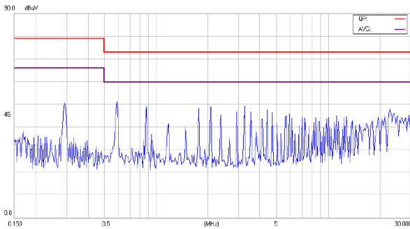
Class A conducted Line test for QB22S5-30
